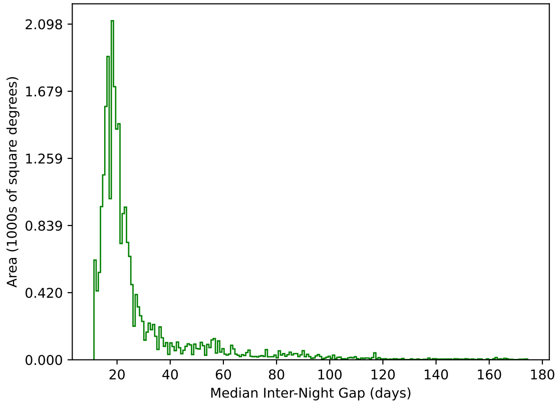
ddf_acor_sf25_lsf40_lsr20_v3.4_10yrs All sky g band: Median Inter-Night Gap
