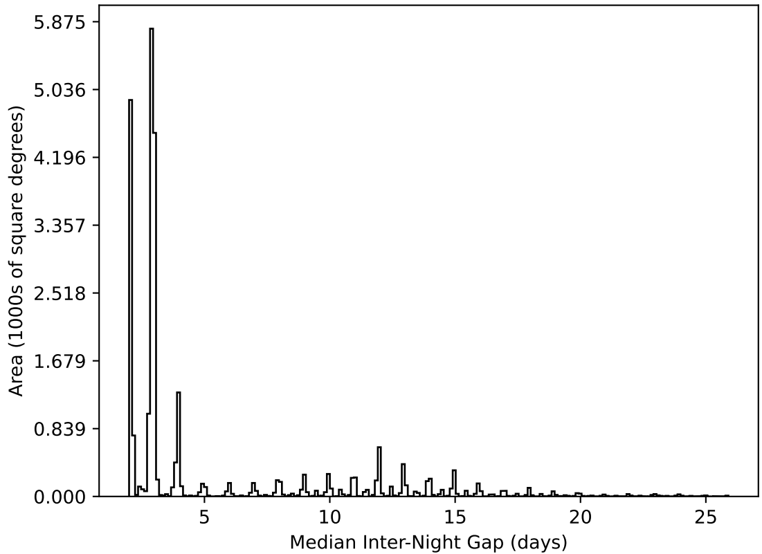
ddf_acor_sf25_lsf40_lsr20_v3.4_10yrs All sky all bands: Median Inter-Night Gap
