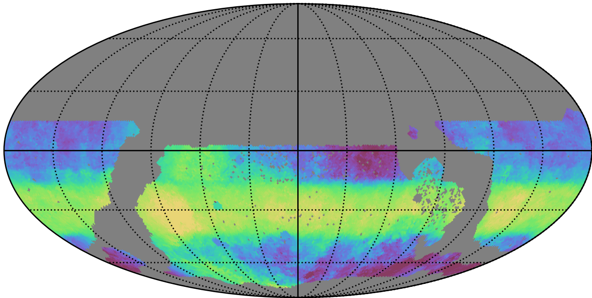
ddf_acor_sf25_lsf40_lsr20_v3.4_10yrs WFD z band: Median HA
