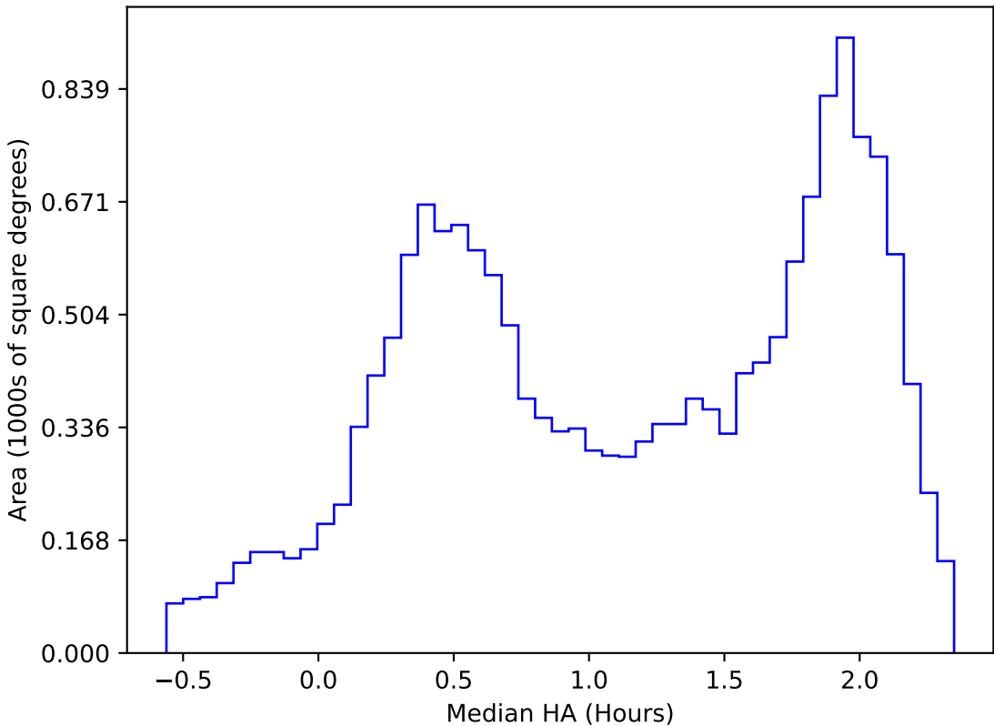
ddf_acor_sf25_lsf40_lsr20_v3.4_10yrs WFD z band: Median HA
