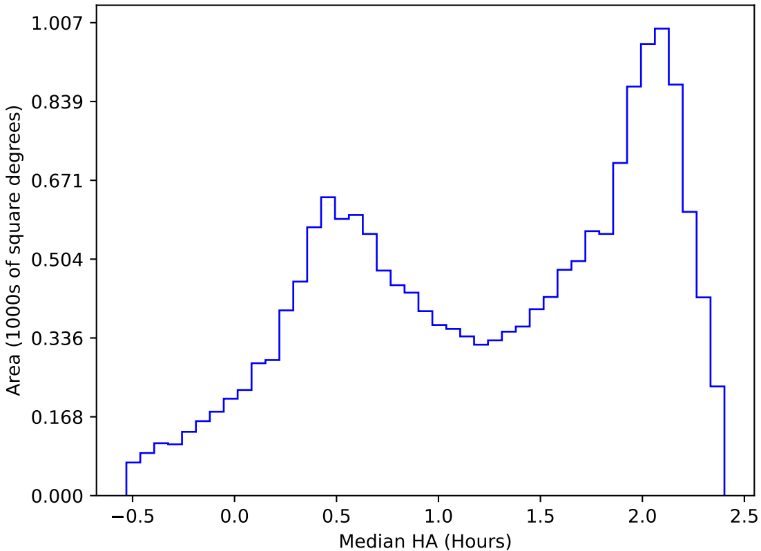
ddf_acor_sf25_lsf40_lsr20_v3.4_10yrs WFD y band: Median HA
