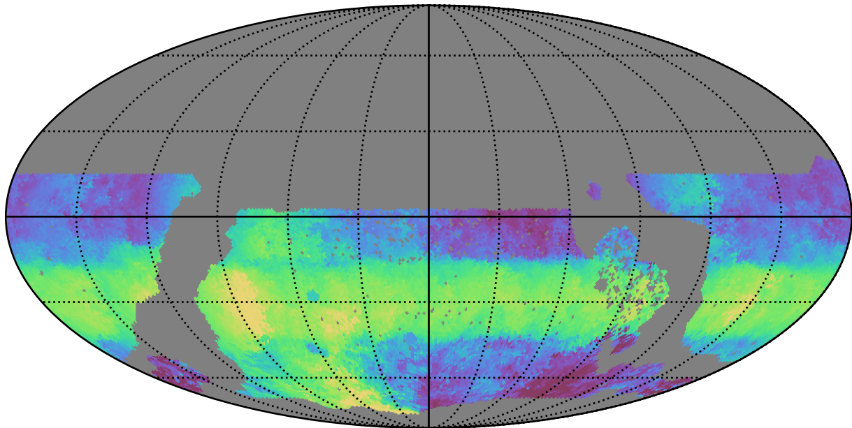
ddf_acor_sf25_lsf40_lsr20_v3.4_10yrs WFD u band: Median HA
