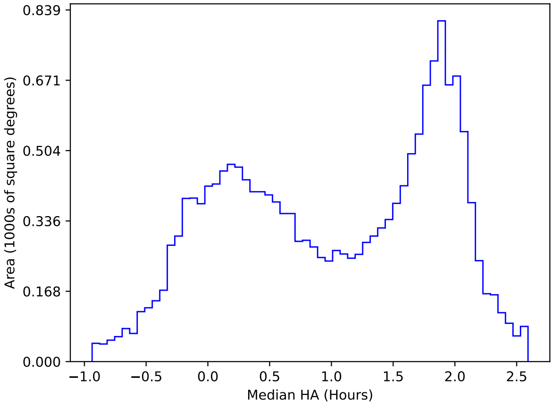
ddf_acor_sf25_lsf40_lsr20_v3.4_10yrs WFD u band: Median HA
