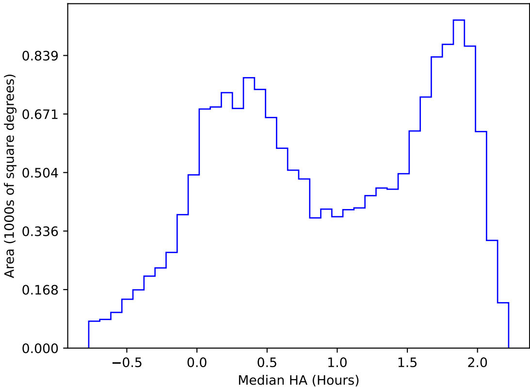
ddf_acor_sf25_lsf40_lsr20_v3.4_10yrs WFD r band: Median HA
