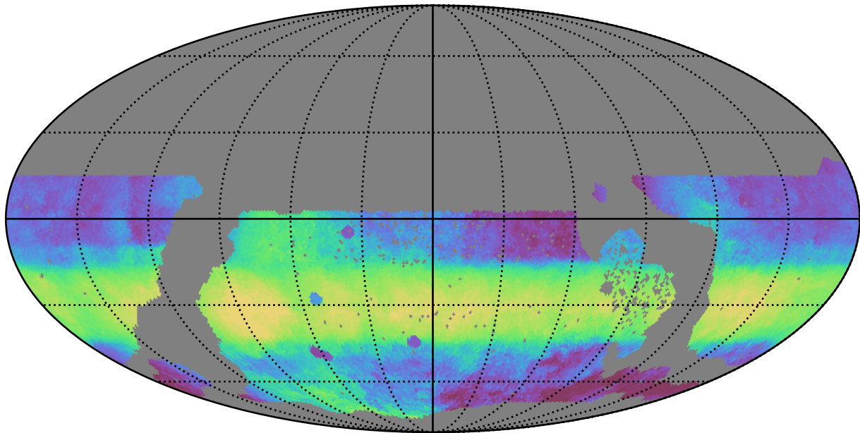
ddf_acor_sf25_lsf40_lsr20_v3.4_10yrs WFD i band: Median HA
