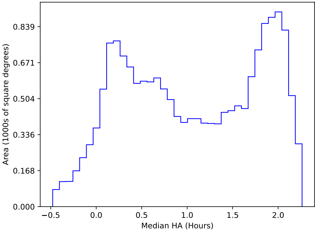
ddf_acor_sf25_lsf40_lsr20_v3.4_10yrs WFD i band: Median HA
