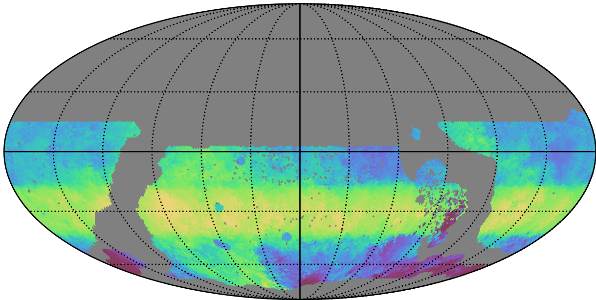
ddf_acor_sf25_lsf40_lsr20_v3.4_10yrs WFD g band: Median HA
