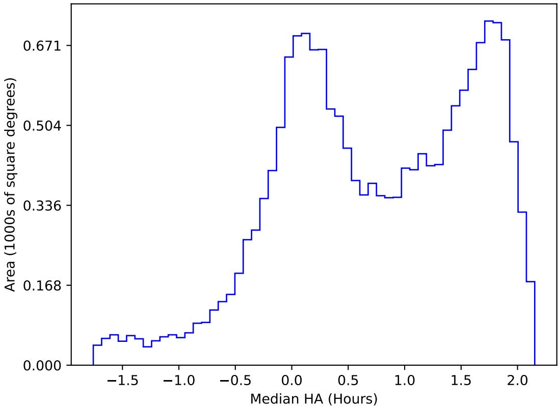
ddf_acor_sf25_lsf40_lsr20_v3.4_10yrs WFD g band: Median HA
