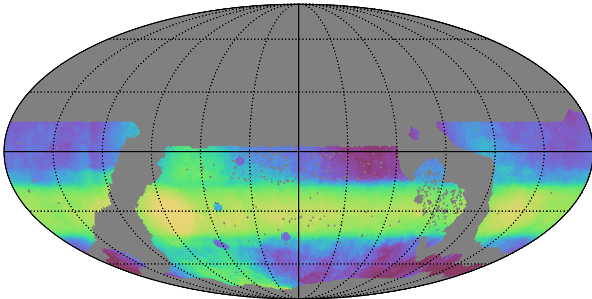
ddf_acor_sf25_lsf40_lsr20_v3.4_10yrs WFD all bands: Median HA
