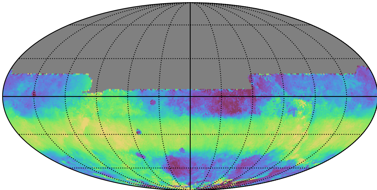
ddf_acor_sf25_lsf40_lsr20_v3.4_10yrs All sky y band: Median HA
