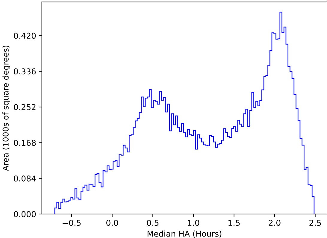
ddf_acor_sf25_ls40_lsr20_v3.4_10yrs All sky y band: Median HA
