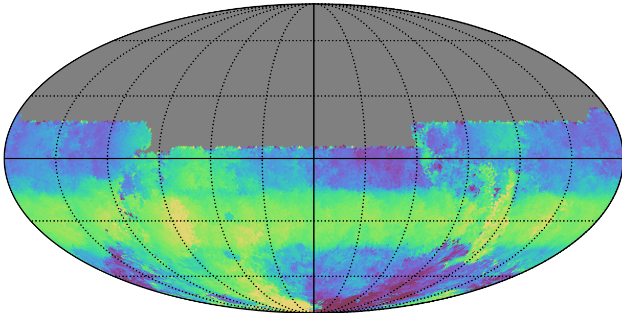
ddf_acor_sf25_lsf40_lsr20_v3.4_10yrs All sky u band: Median HA
