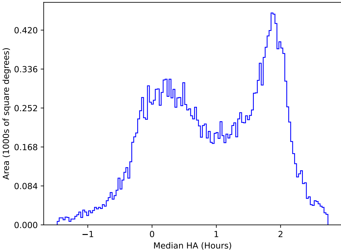
ddf_acor_sf25_lsf40_lsr20_v3.4_10yrs All sky u band: Median HA
