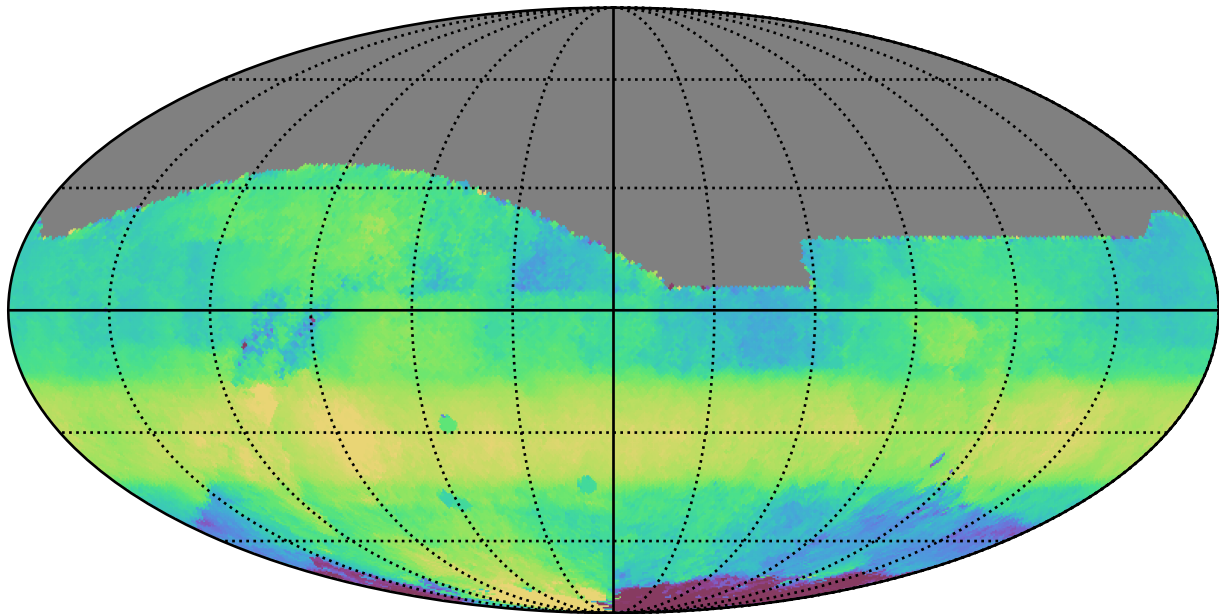
ddf_acor_sf25_lsf40_lsr20_v3.4_10yrs All sky r band: Median HA
