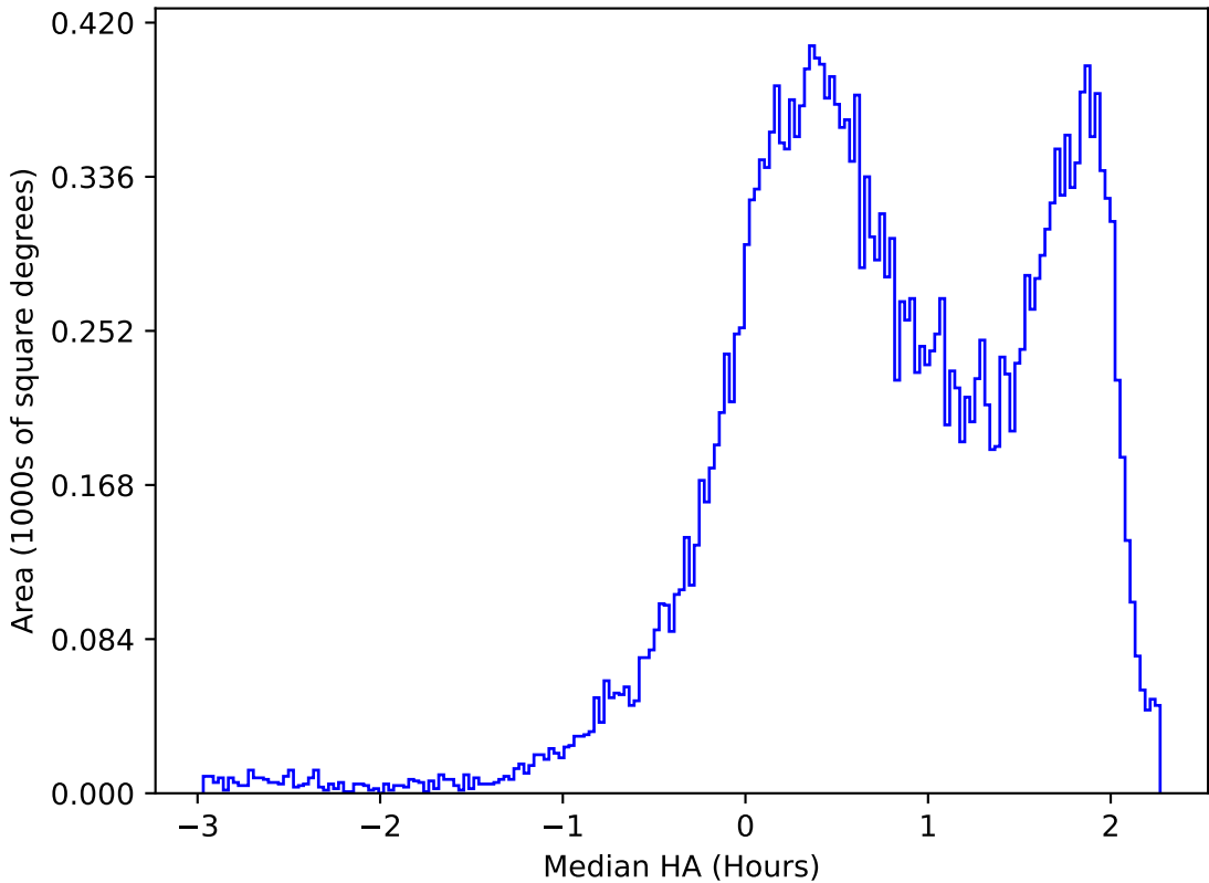
ddf_acor_sf25_lsf40_lsr20_v3.4_10yrs All sky r band: Median HA
