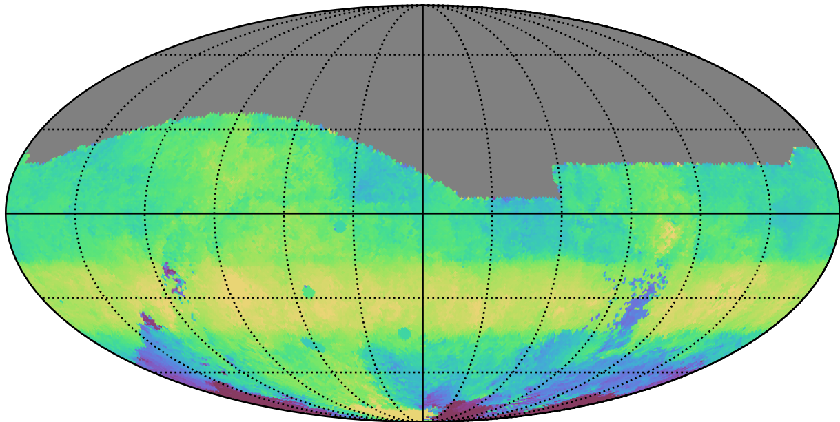
ddf_acor_sf25_lsf40_lsr20_v3.4_10yrs All sky g band: Median HA
