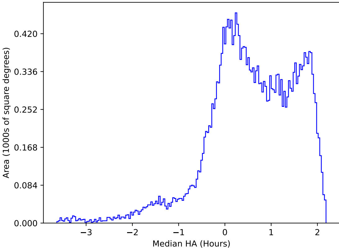
ddf_acor_sf25_lsf40_lsr20_v3.4_10yrs All sky g band: Median HA
