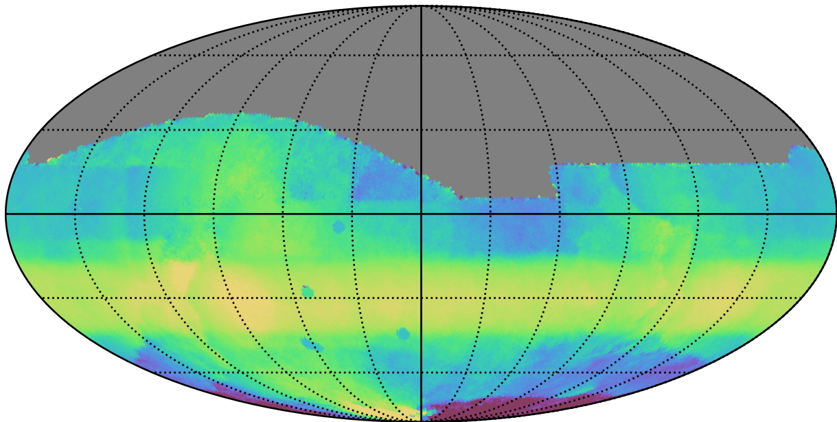
ddf_acor_sf25_lsf40_lsr20_v3.4_10yrs All sky all bands: Median HA
