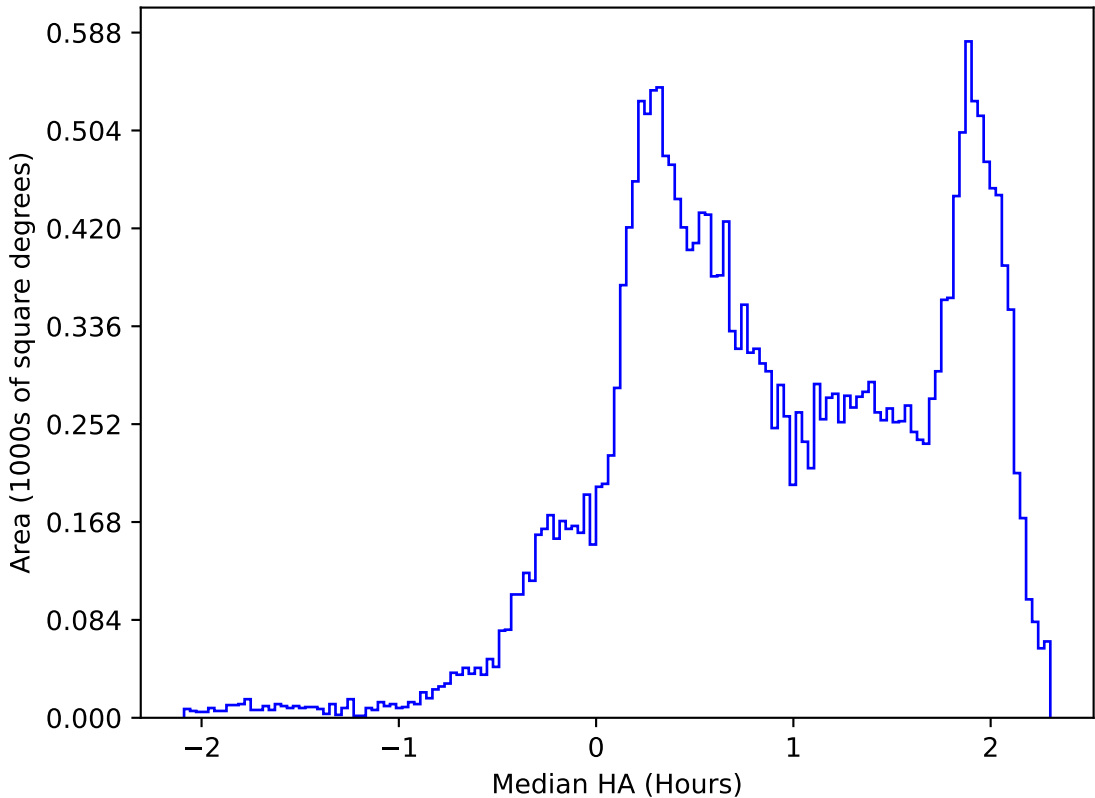
ddf_acor_sf25_lsf40_lsr20_v3.4_10yrs All sky all bands: Median HA
