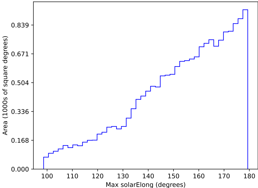
ddf_acor_sf25_lsf40_lsr20_v3.4_10yrs WFD y band: Max solarElong
