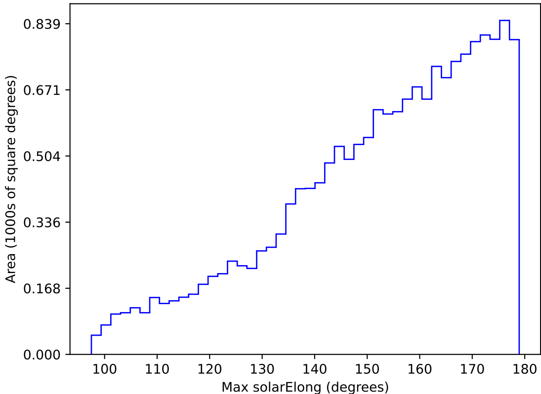
ddf_acor_sf25_lsf40_lsr20_v3.4_10yrs WFD u band: Max solarElong
