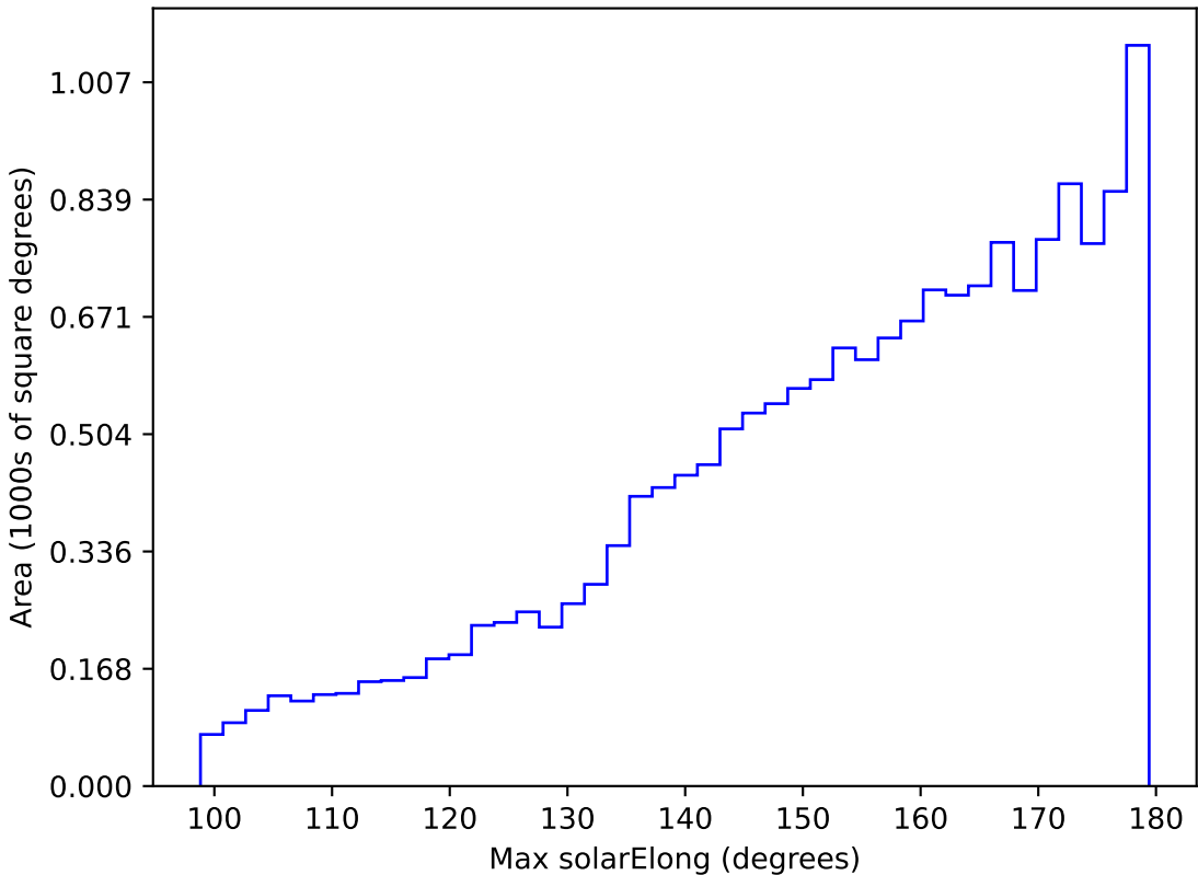
ddf_acor_sf25_lsf40_lsr20_v3.4_10yrs WFD r band: Max solarElong
