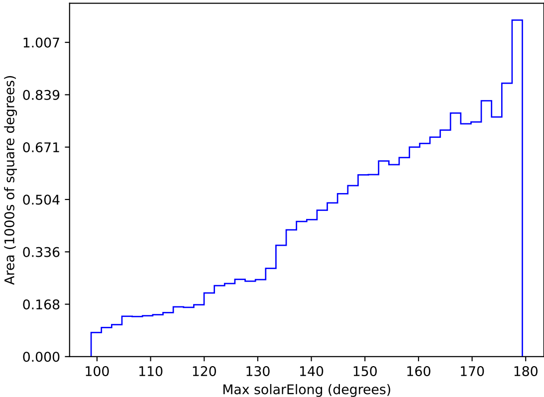
ddf_acor_sf25_lsf40_lsr20_v3.4_10yrs WFD i band: Max solarElong
