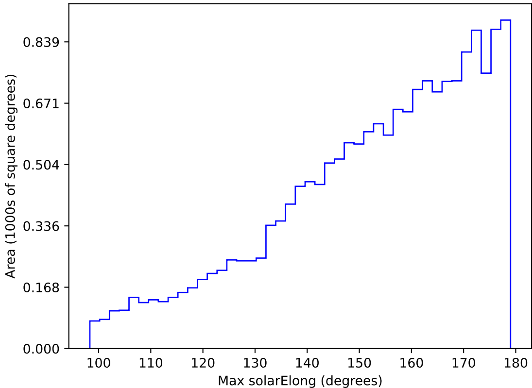
ddf_acor_sf25_lsf40_lsr20_v3.4_10yrs WFD g band: Max solarElong
