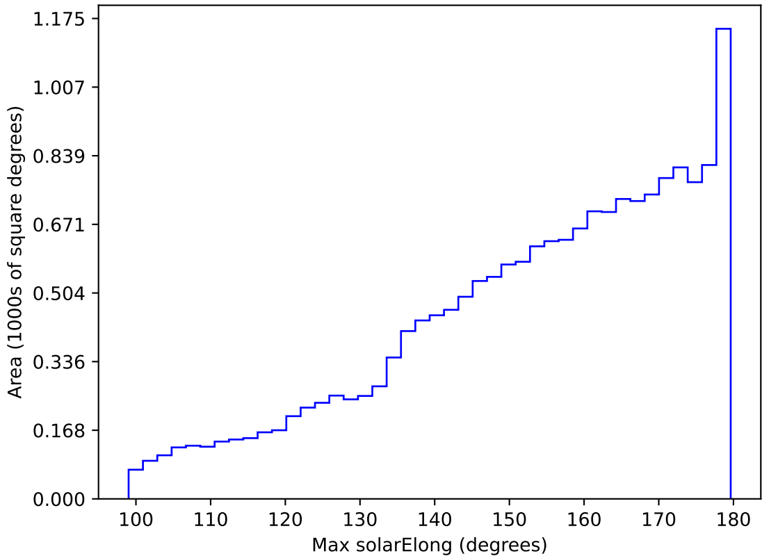
ddf_acor_sf25_lsf40_lsr20_v3.4_10yrs WFD all bands: Max solarElong
