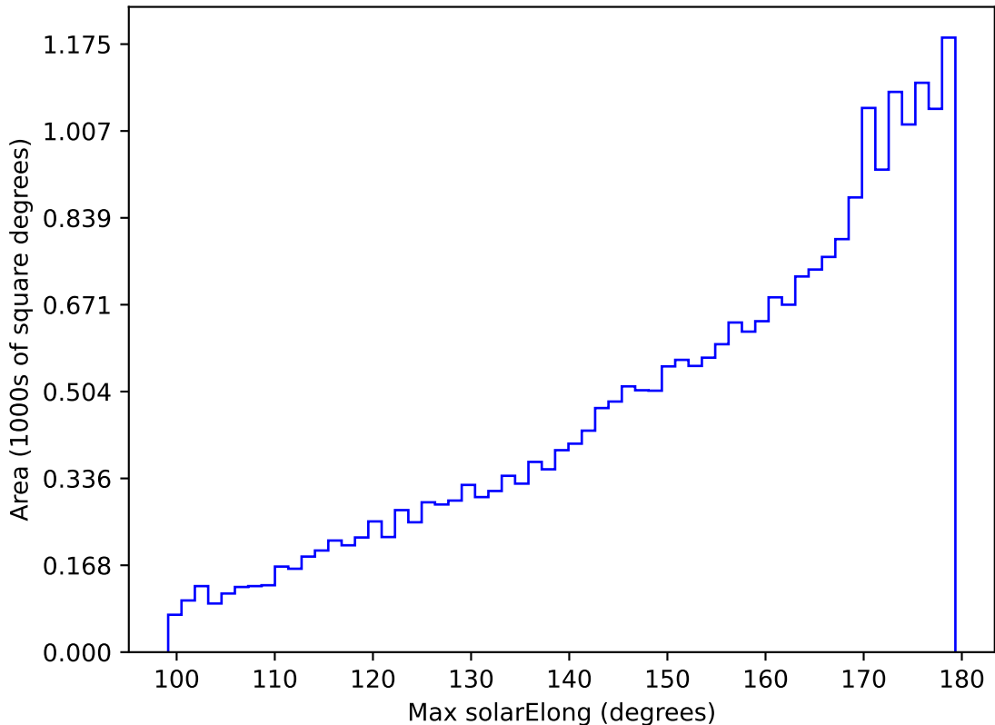
ddf_acor_sf25_lsf40_lsr20_v3.4_10yrs All sky z band: Max solarElong
