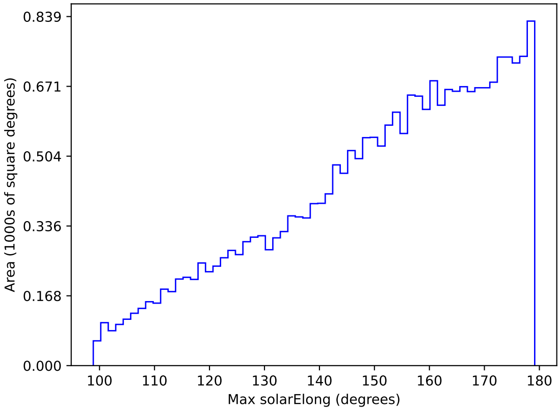
ddf_acor_sf25_lsf40_lsr20_v3.4_10yrs All sky y band: Max solarElong
