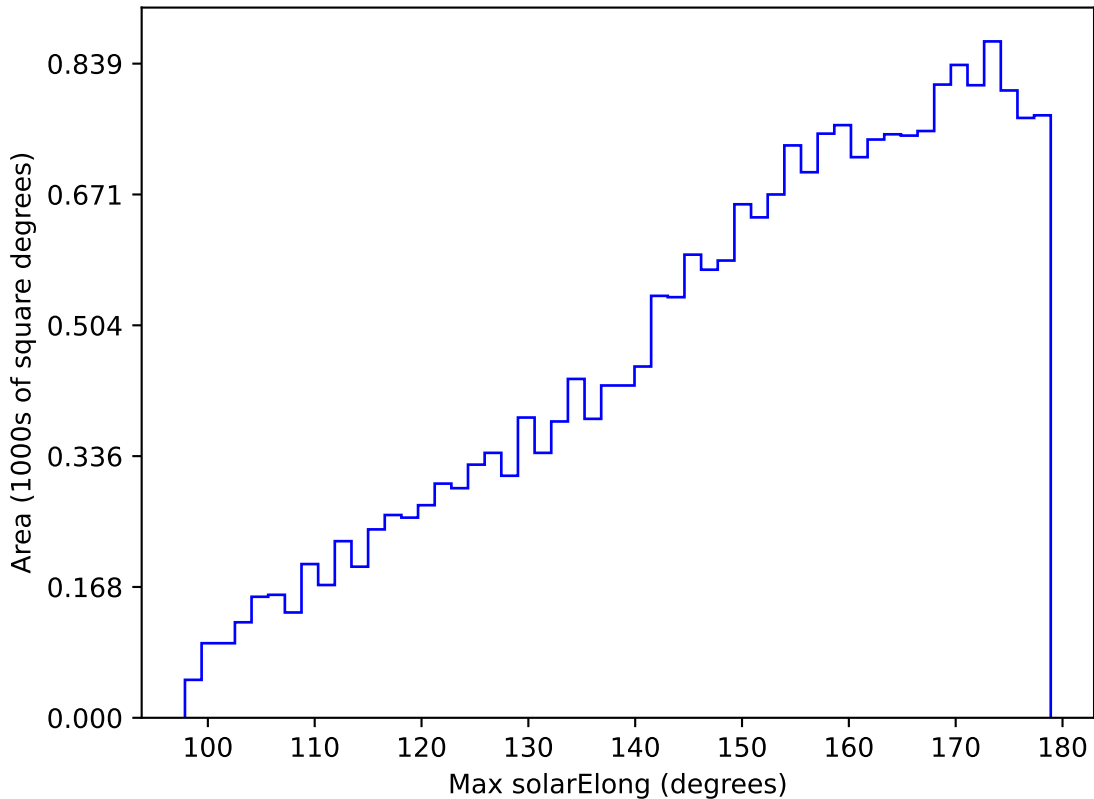
ddf_acor_sf25_lsf40_lsr20_v3.4_10yrs All sky u band: Max solarElong
