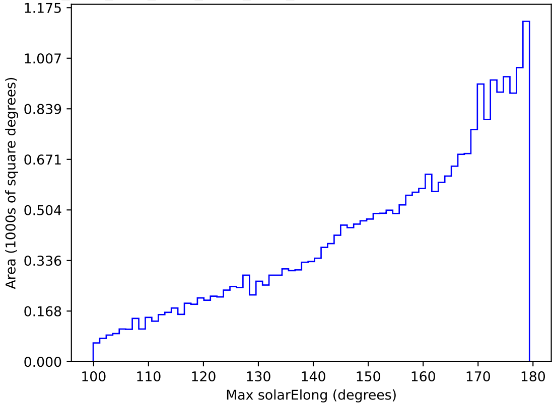
ddf_acor_sf25_lsf40_lsr20_v3.4_10yrs All sky r band: Max solarElong
