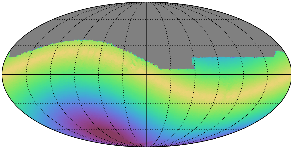
ddf_acor_sf25_lsf40_lsr20_v3.4_10yrs All sky i band: Max solarElong
