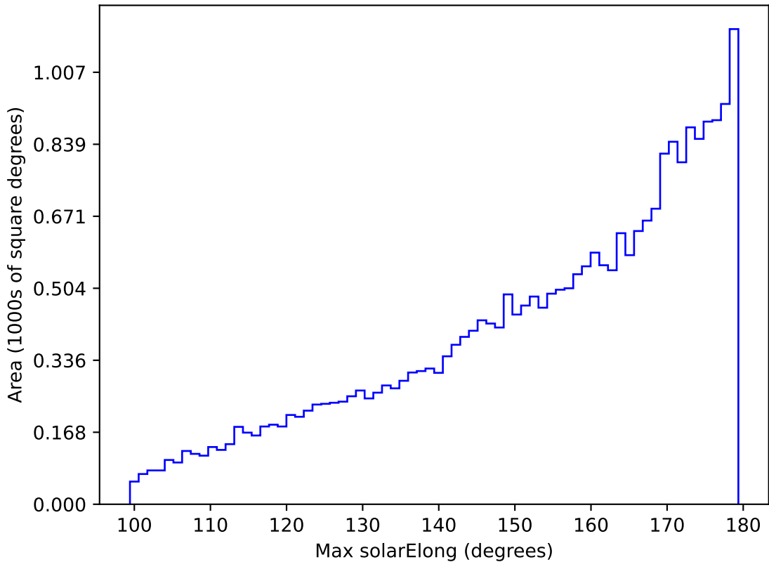
ddf_acor_sf25_lsf40_lsr20_v3.4_10yrs All sky i band: Max solarElong
