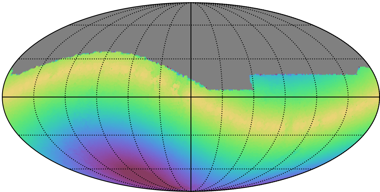
ddf_acor_sf25_lsf40_lsr20_v3.4_10yrs All sky g band: Max solarElong
