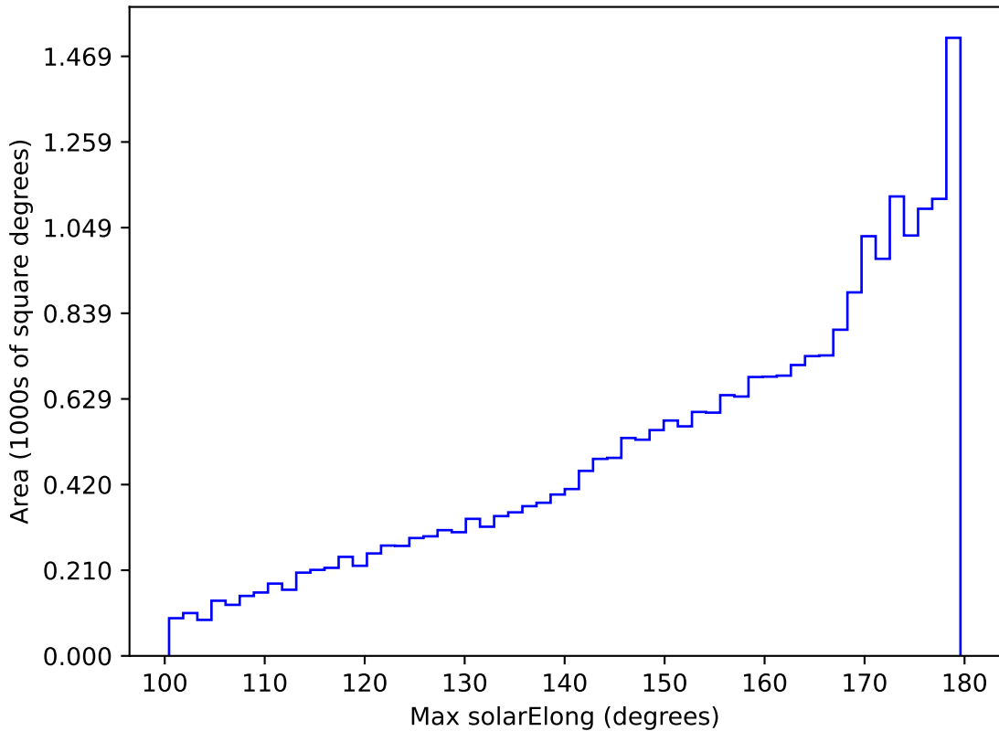
ddf_acor_sf25_lsf40_lsr20_v3.4_10yrs All sky all bands: Max solarElong
