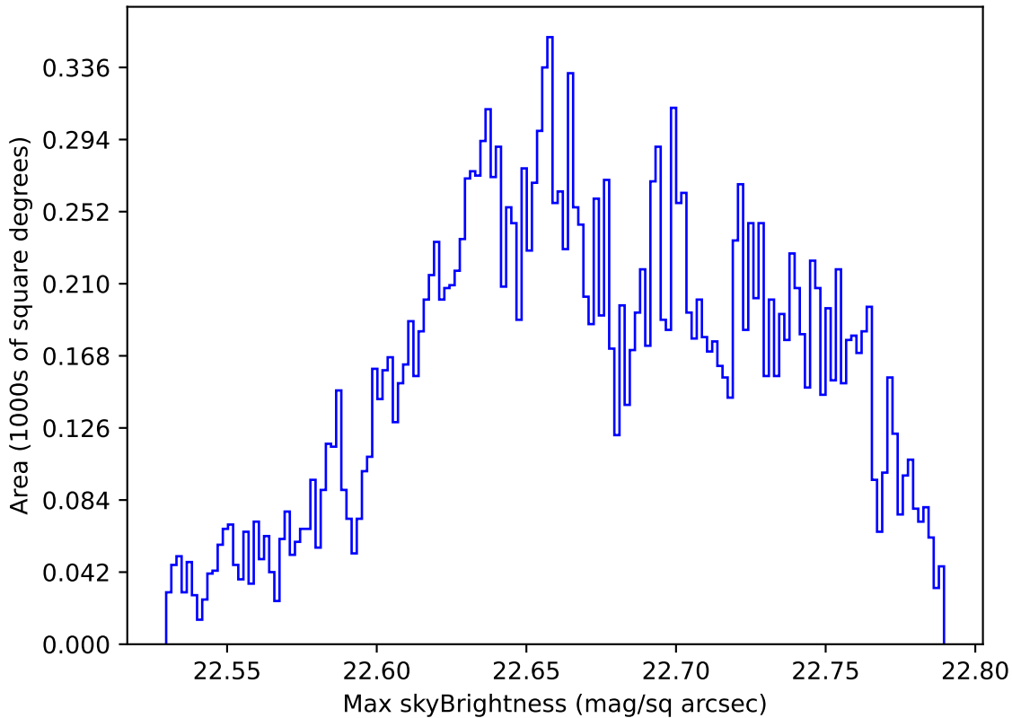
ddf_acor_sf25_lsf40_lsr20_v3.4_10yrs Yr 1 u band: Max skyBrightness
