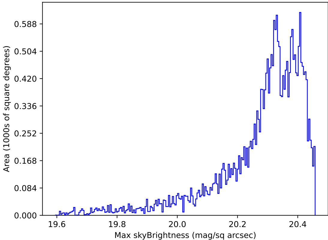
ddf_acor_sf25_lsf40_lsr20_v3.4_10yrs Yr 1 i band: Max skyBrightness
