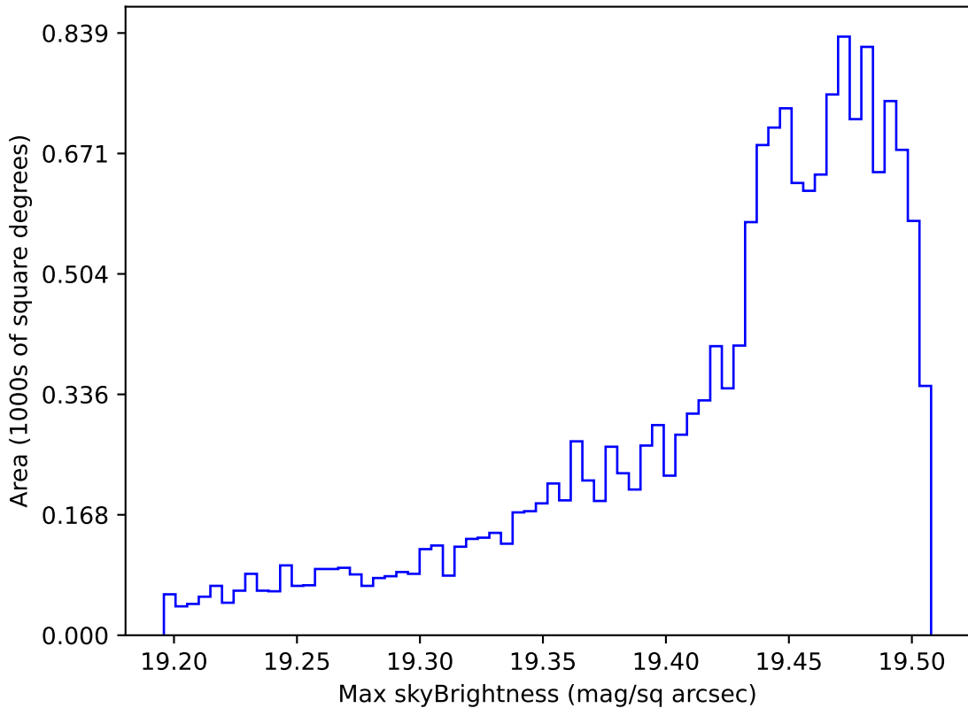
ddf_acor_sf25_lsf40_lsr20_v3.4_10yrs WFD z band: Max skyBrightness
