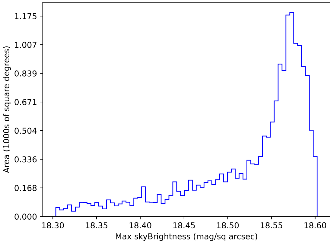
ddf_acor_sf25_lsf40_lsr20_v3.4_10yrs WFD y band: Max skyBrightness
