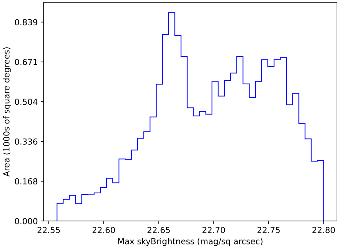
ddf_acor_sf25_lsf40_lsr20_v3.4_10yrs WFD u band: Max skyBrightness
