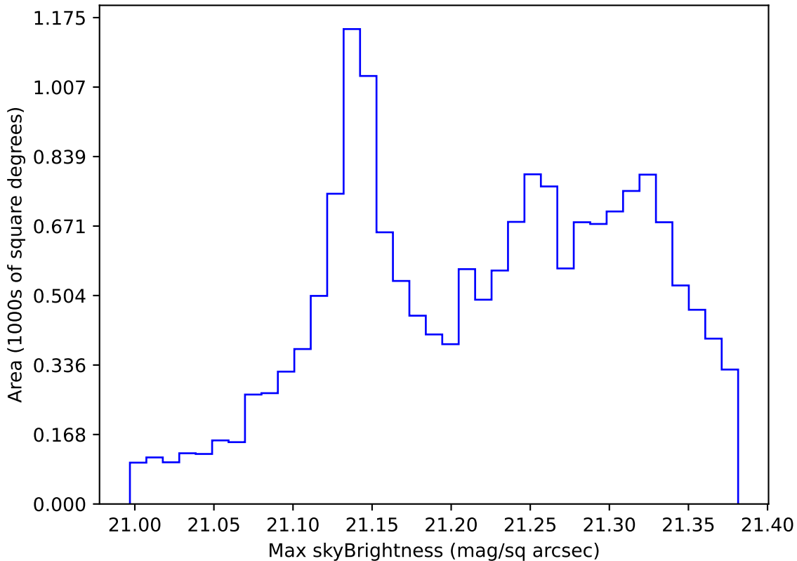
ddf_acor_sf25_lsf40_lsr20_v3.4_10yrs WFD r band: Max skyBrightness
