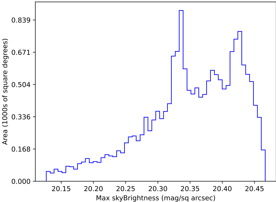
ddf_acor_sf25_lsf40_lsr20_v3.4_10yrs WFD i band: Max skyBrightness
