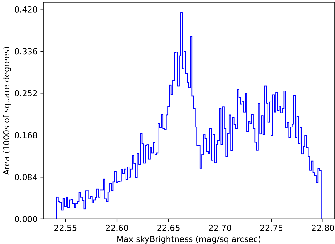
ddf_acor_sf25_lsf40_lsr20_v3.4_10yrs All sky u band: Max skyBrightness
