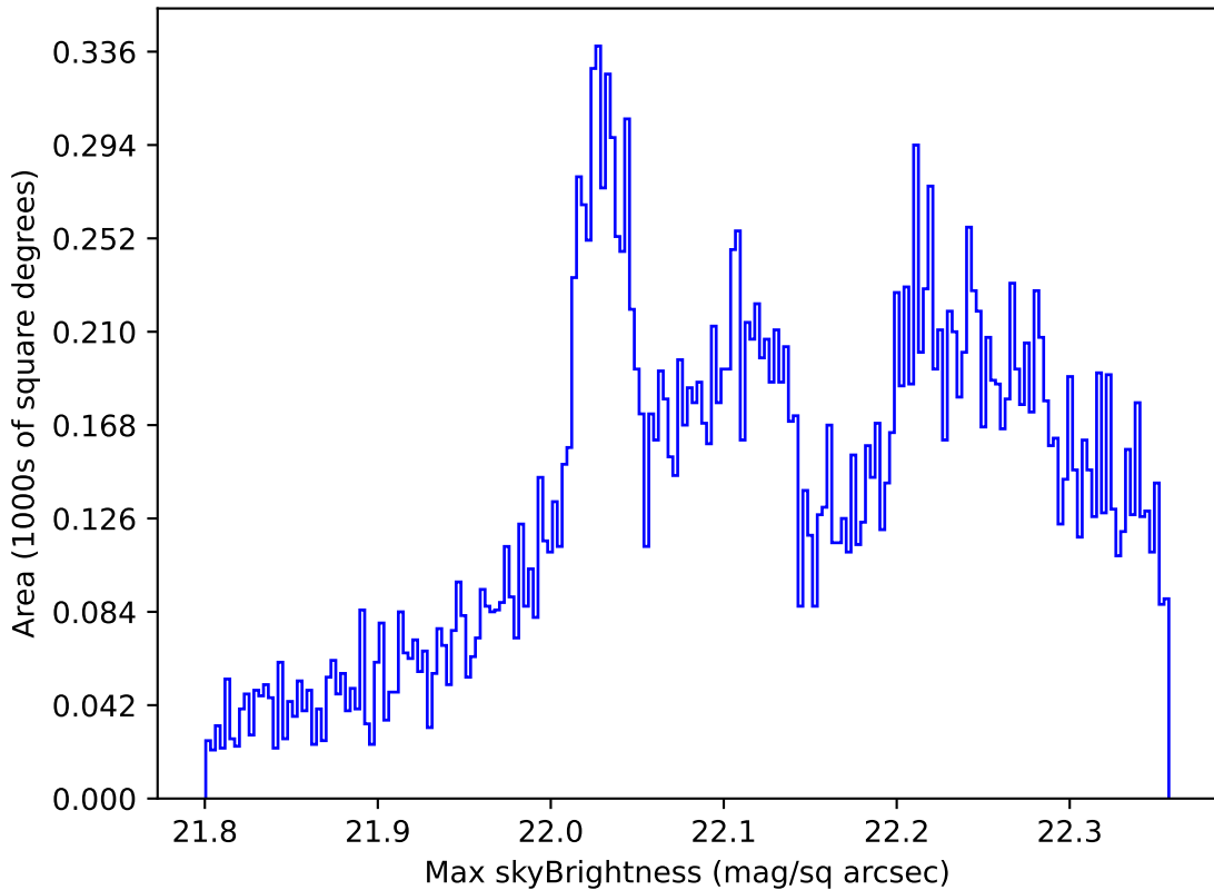
ddf_acor_sf25_lsf40_lsr20_v3.4_10yrs All sky g band: Max skyBrightness
