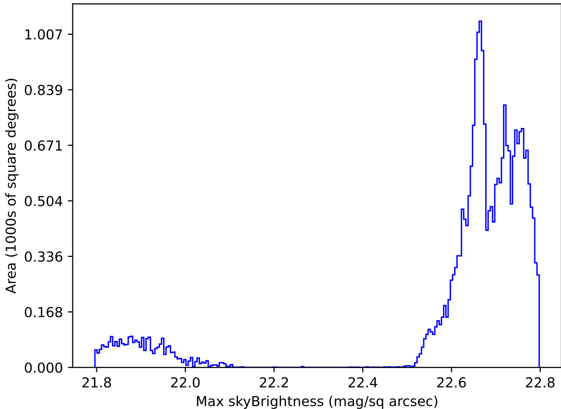
ddf_acor_sf25_lsf40_lsr20_v3.4_10yrs All sky all bands: Max skyBrightness
