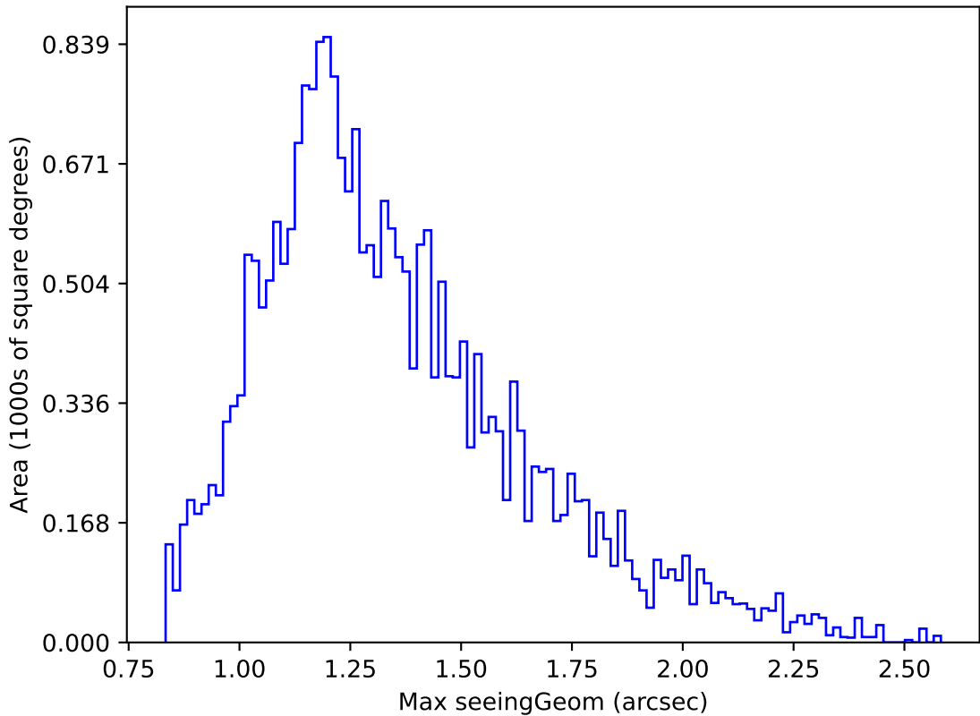
ddf_acor_sf25_lsf40_lsr20_v3.4_10yrs Yr 1 r band: Max seeingGeom
