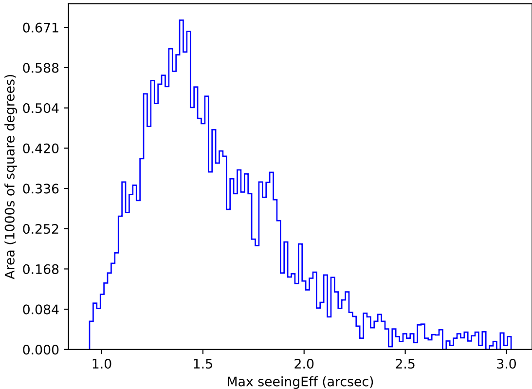
ddf_acor_sf25_lsf40_lsr20_v3.4_10yrs Yr 1 u band: Max seeingEff
