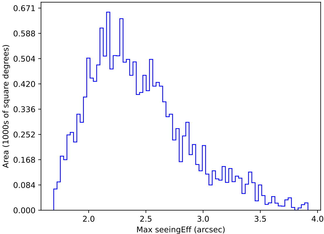
ddf_acor_sf25_lsf40_lsr20_v3.4_10yrs WFD u band: Max seeingEff
